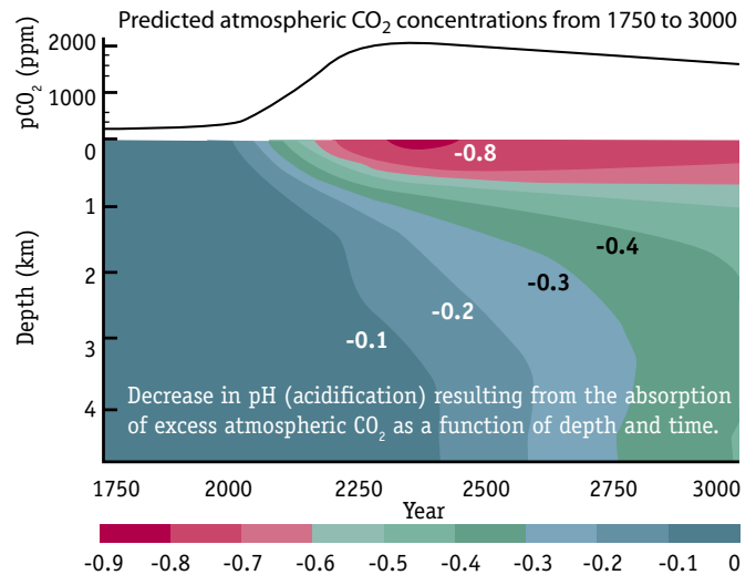
\Delta\text{pH} © Caldeira & Wickett (2003, Science)
