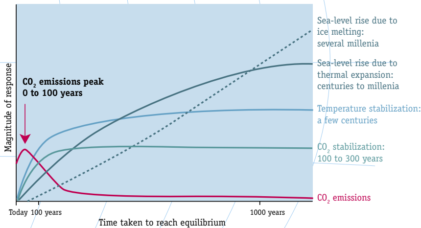
CO 2 concentration, temperature and sea level continue to rise long after emissions are reduced.
