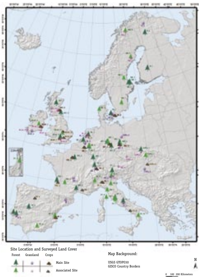
Flux/Ecology sites in the CarboEurope-IP.
